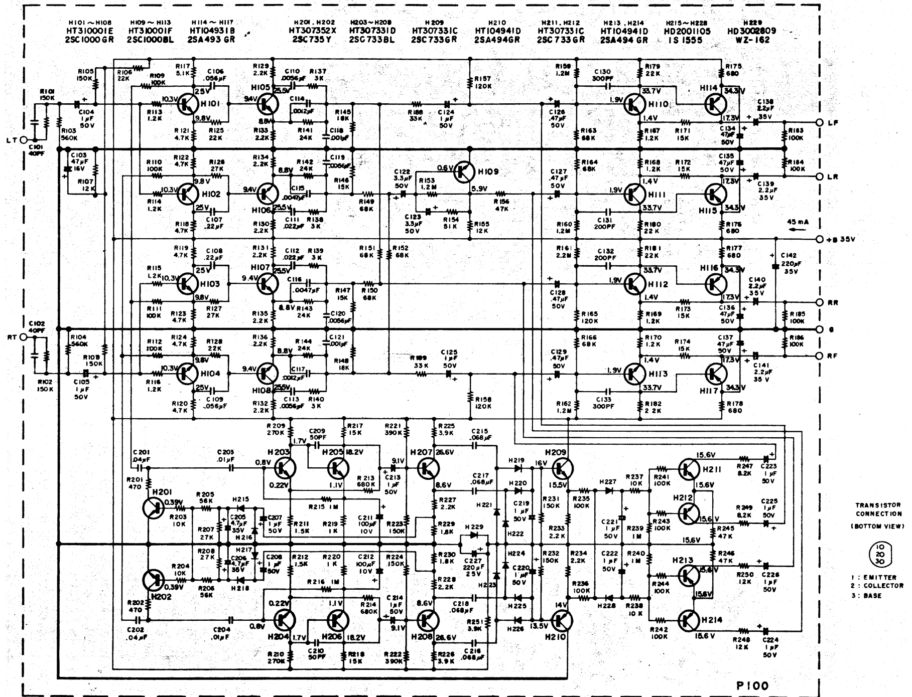
Marantz SQA 1 - Schematic Diagram
